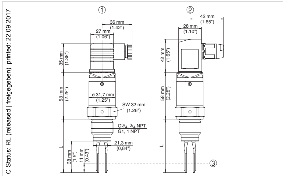
Fig. 33: LEVEL SWITCH 8110, version standard - Filetage G \frac{3}{4} , G1 / \frac{3}{4} NPT, 1 NPT
