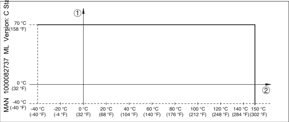
Fig. 31: Dependency ambient temperature to process temperature
