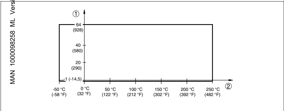
Fig. 26: Process temperature - Process pressure with switch position 0.7 g/cm³ (sensitivity switch)
