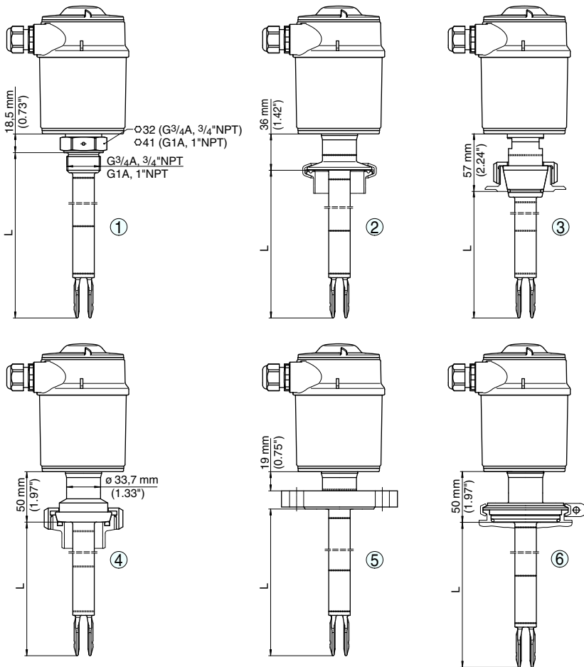
Abb. 29: LEVEL SWITCH 8112
