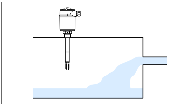
Fig. 8: Inflowing medium
