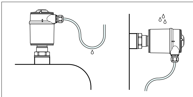
Fig. 6: Measures against moisture penetration
