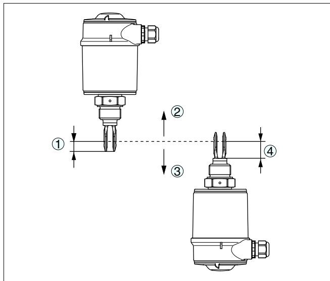
Fig. 2: Montage vertical
