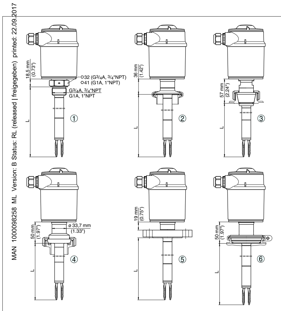
Fig. 27: LEVEL SWITCH 8112
