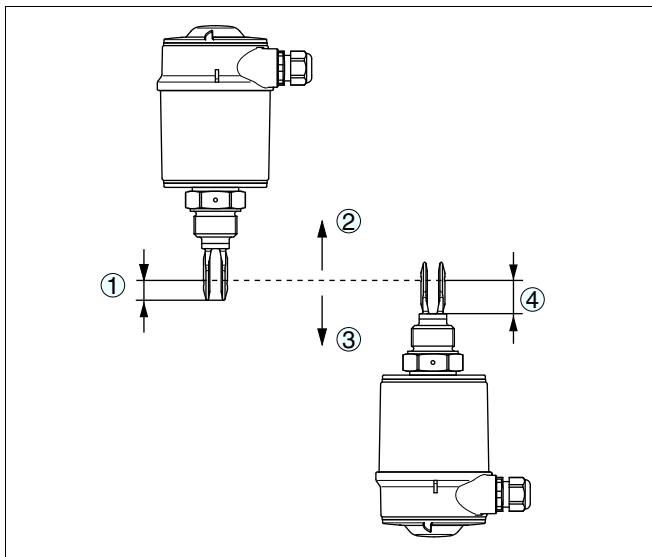
Fig. 2: Installation vertical
