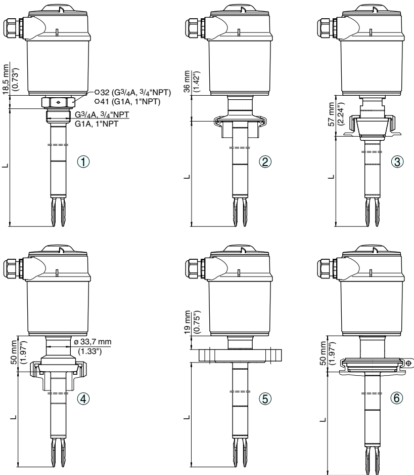
Fig. 29: LEVEL SWITCH 8112
