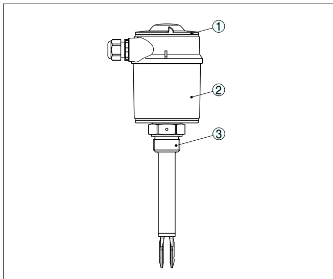
Fig. 1: LEVEL SWITCH 8112 - with plastic housing
