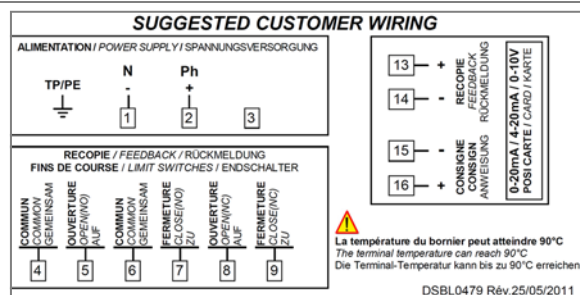
3004 (25-75 NM)/3004 (100-300 NM) multivolt POSI
